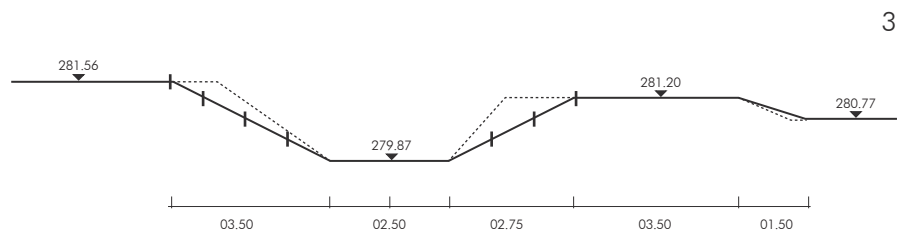
Rosal stream - bank reshaping and reprofiling Cross sections
